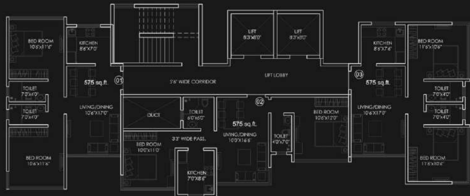
Proposed Residential Building at Byculla
